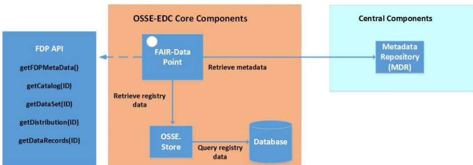
Figure 1. Extended OSSE-Architecture.
